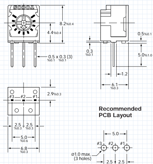
GF063V1 V1 Terminal Style, Cross-Slot, Side Adjust
