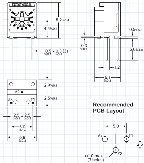
GF063V1 V1 Terminal Style, Cross-Slot, Side Adjust
