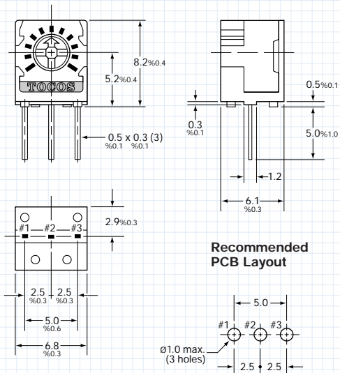
GF063V V & V-3* Terminal Styles, Cross-Slot, Side Adjust
