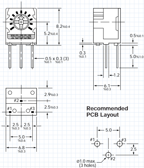
GF063V V & V-3* Terminal Styles, Cross-Slot, Side Adjust
